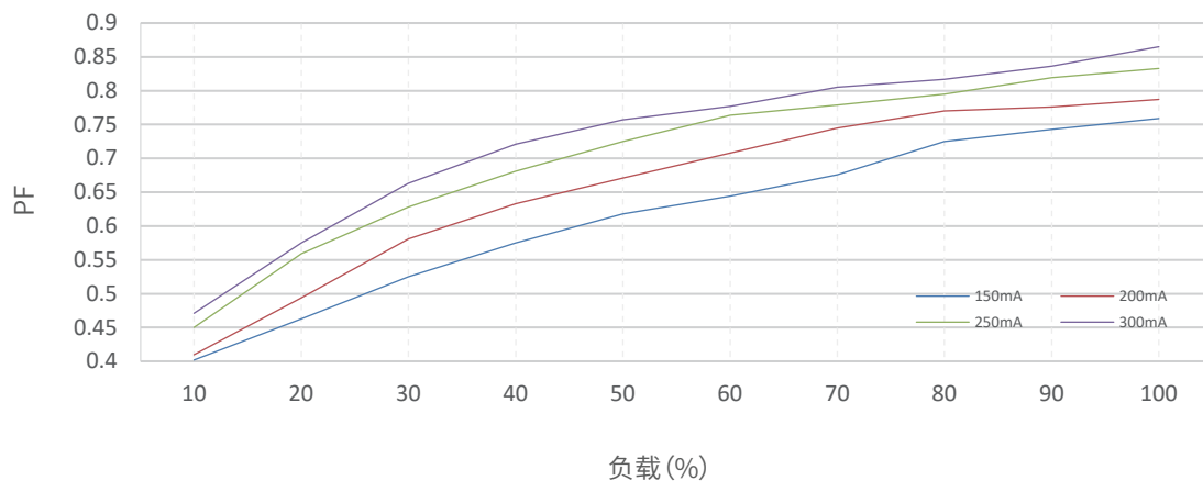
功率因数VS负载@230Vac
