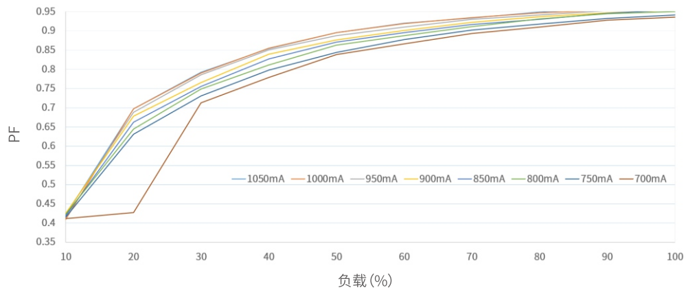
Power Factor VS @Load 230Vac
