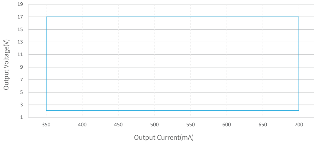
Operating Window
