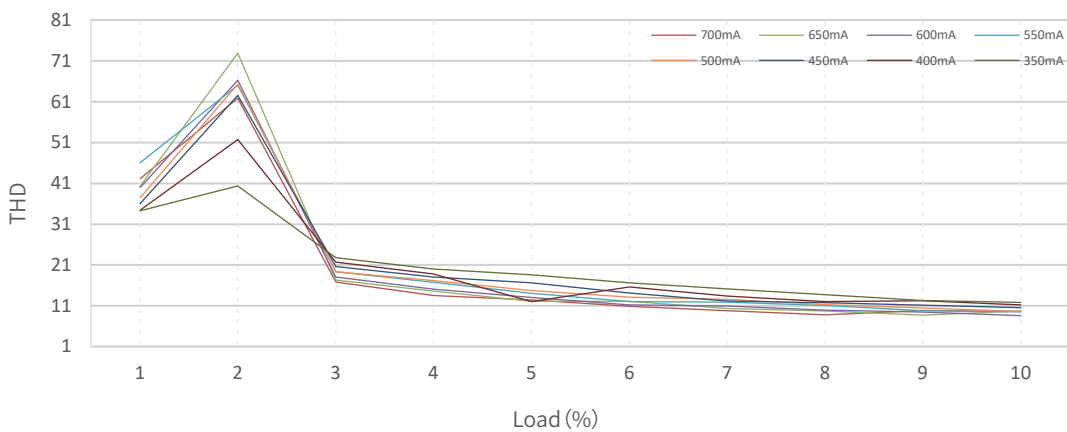
THD VS @Load 230Vac
