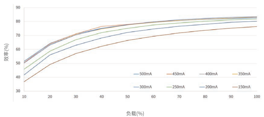
效率VS负载@230Vac
