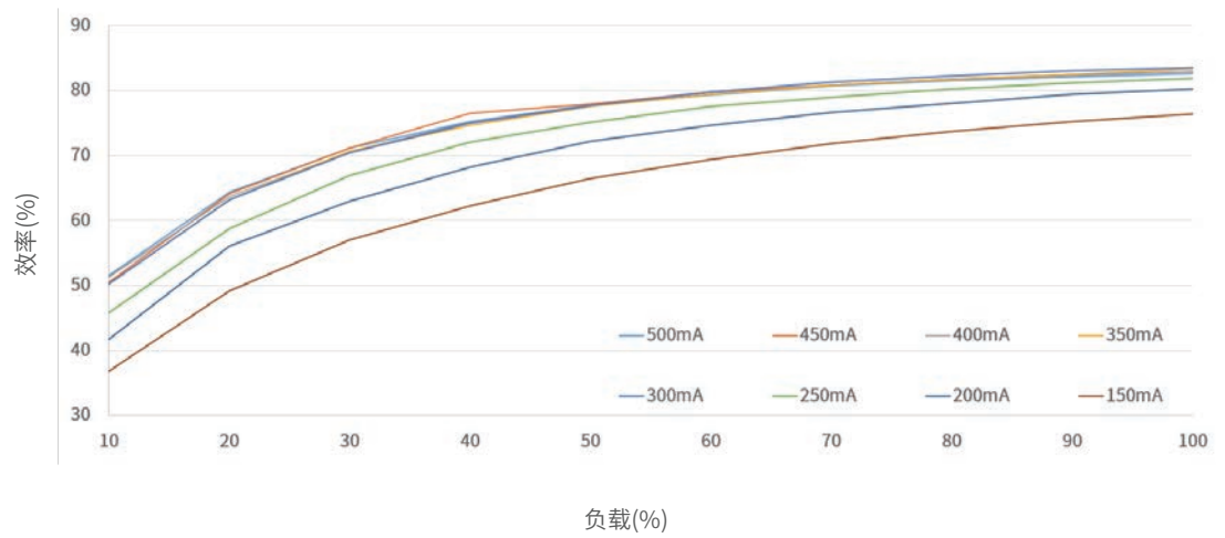
效率VS负载@230Vac
