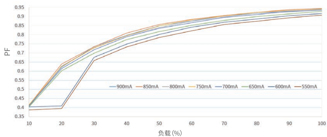
功率因数VS负载@230Vac
