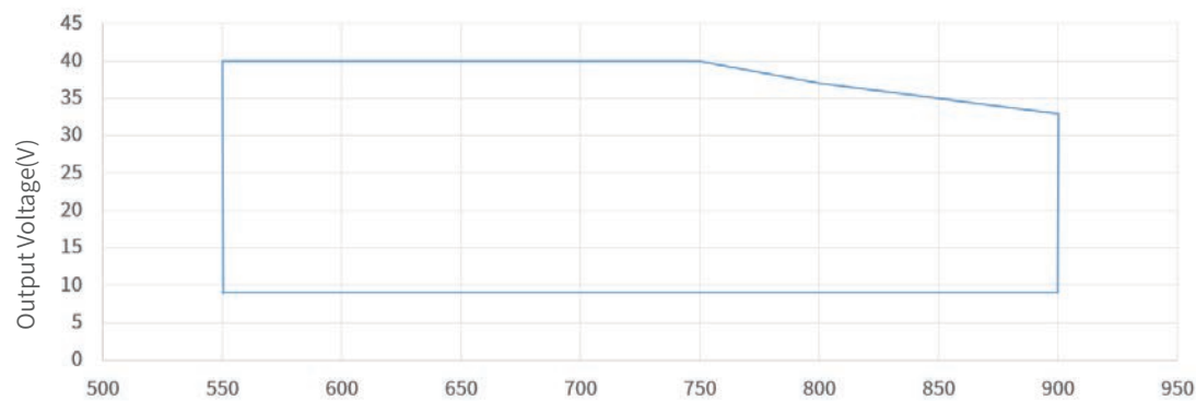
Operating Window
