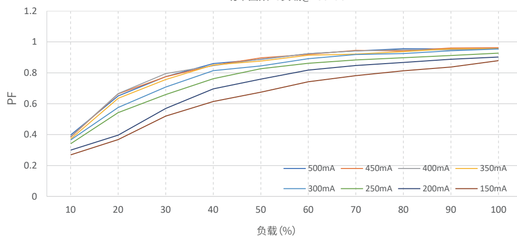
功率因数VS负载@230Vac
