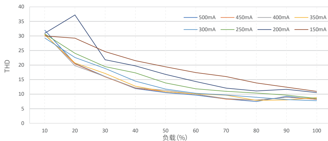
谐波VS负载@230Vac
