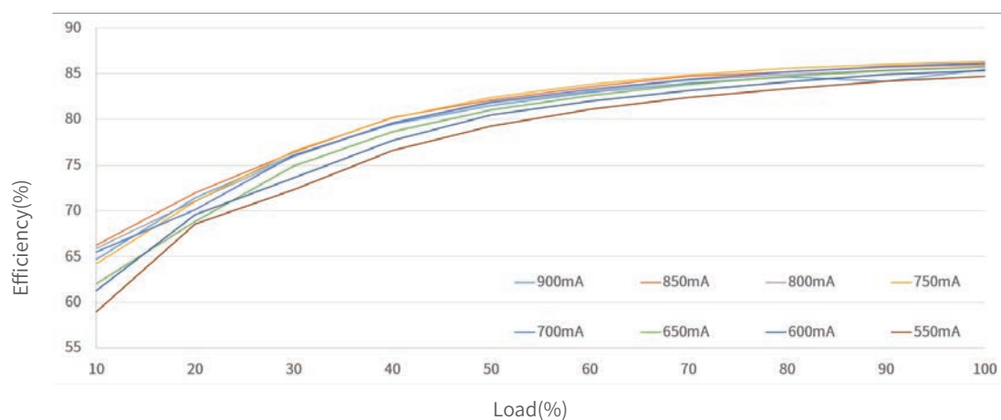
Efficiency VS Load@230Vac
