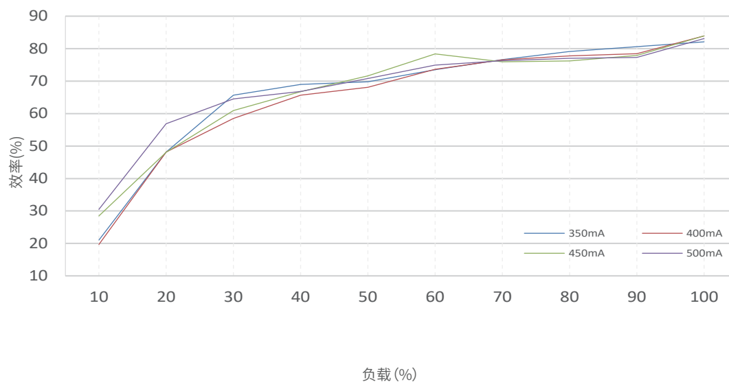
效率VS负载@230Vac
