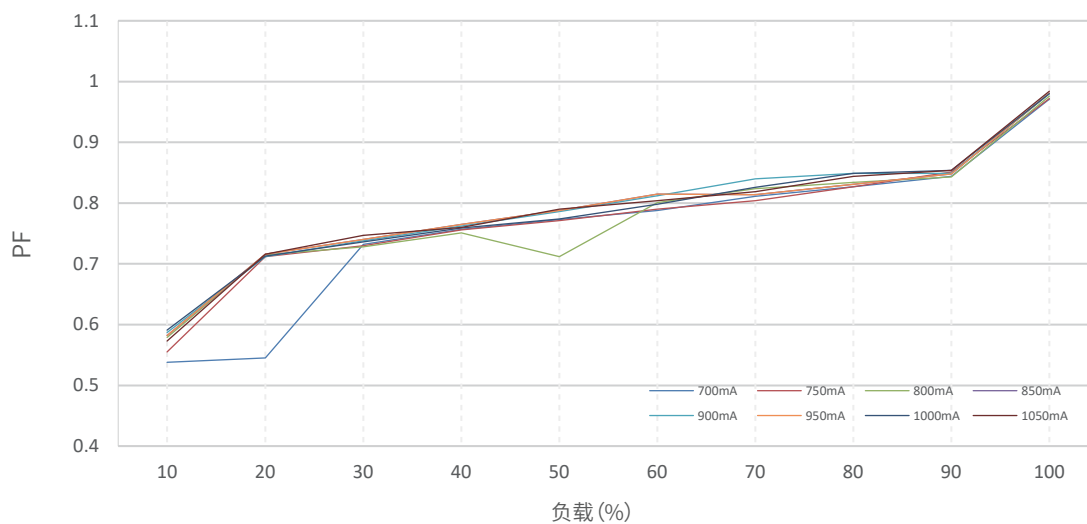
功率因数VS负载@230Vac
